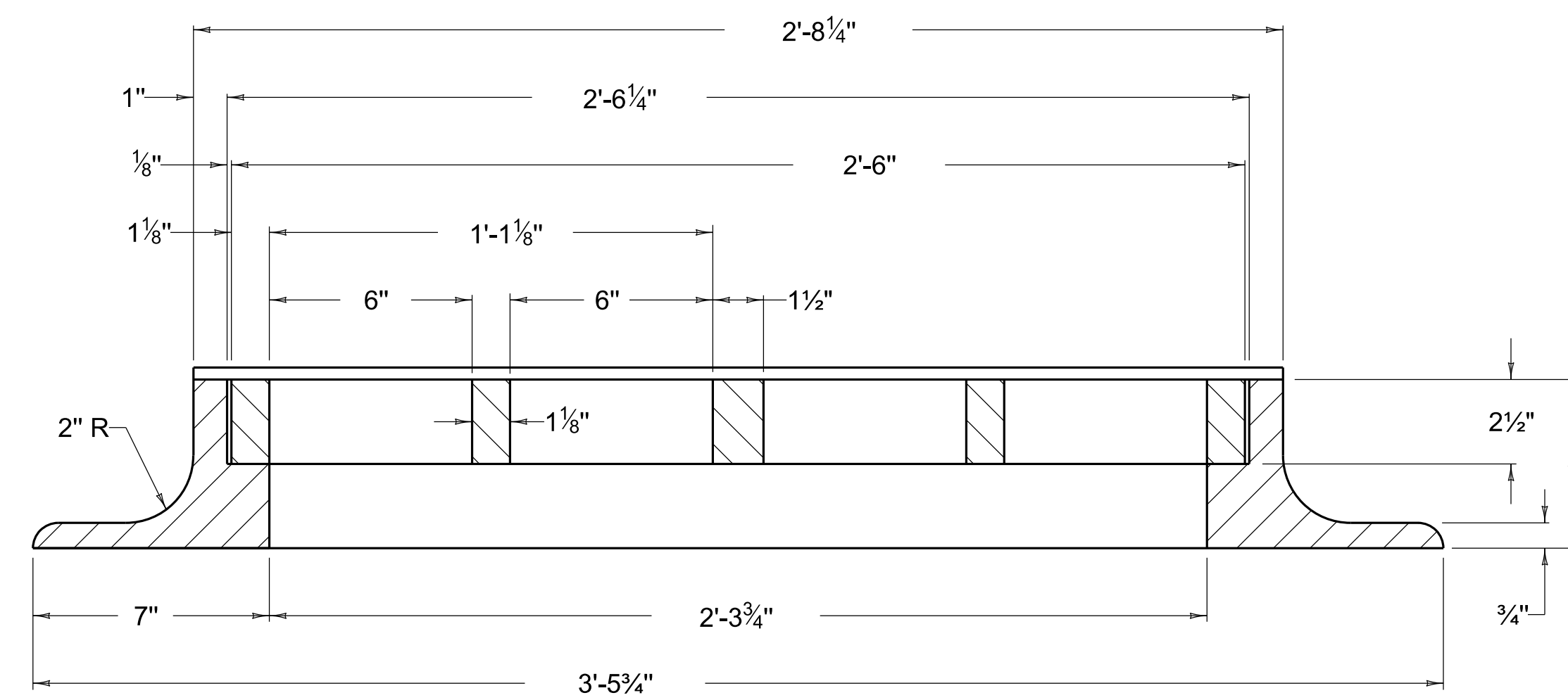
SECTIONAL VIEW OF FRAME AND GRATE
